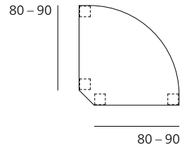
640/10 System panels Extension leaf Corner element 90°
