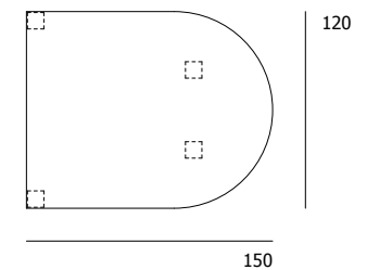
640/81 System panels End table top panel Semi-oval
