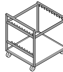
246/75 Four-wheeled trolley to take five folding tables 540/15 (table depth 75 cm)
